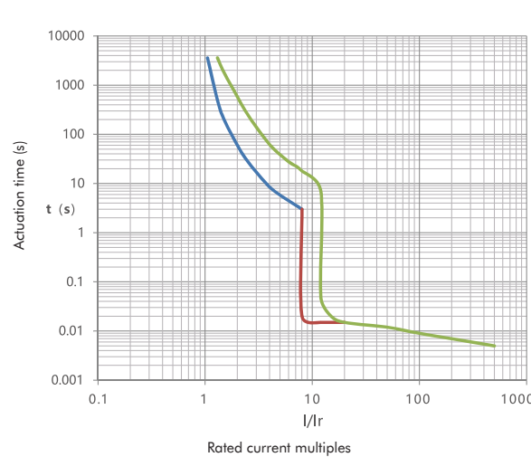
Tripping curve
