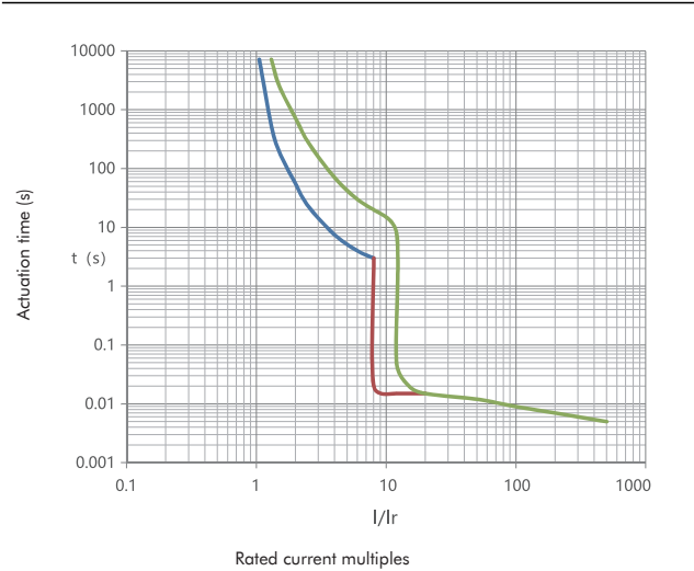
Tripping curve
